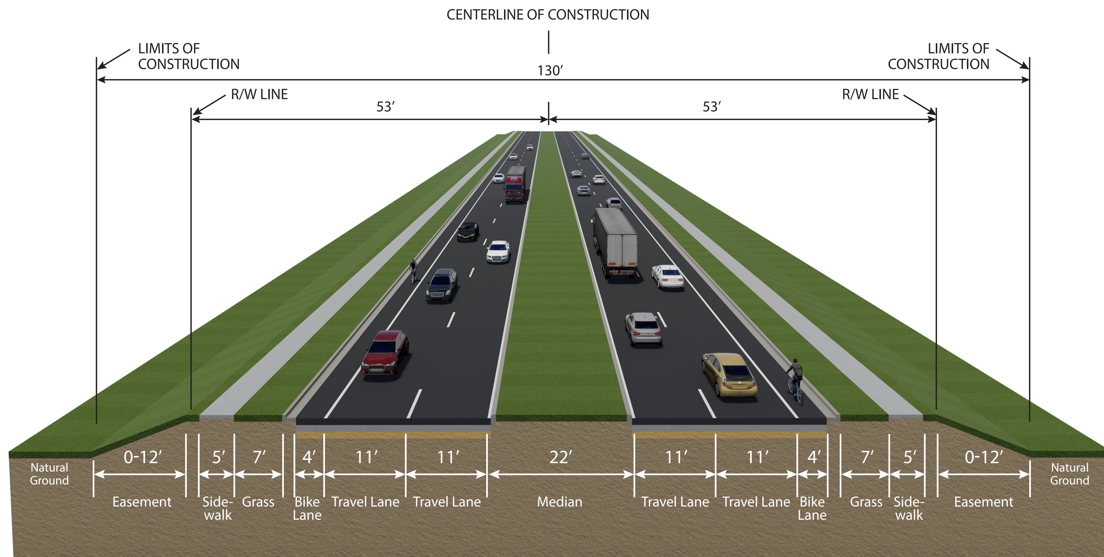
Typical Section - Except on Bridge
