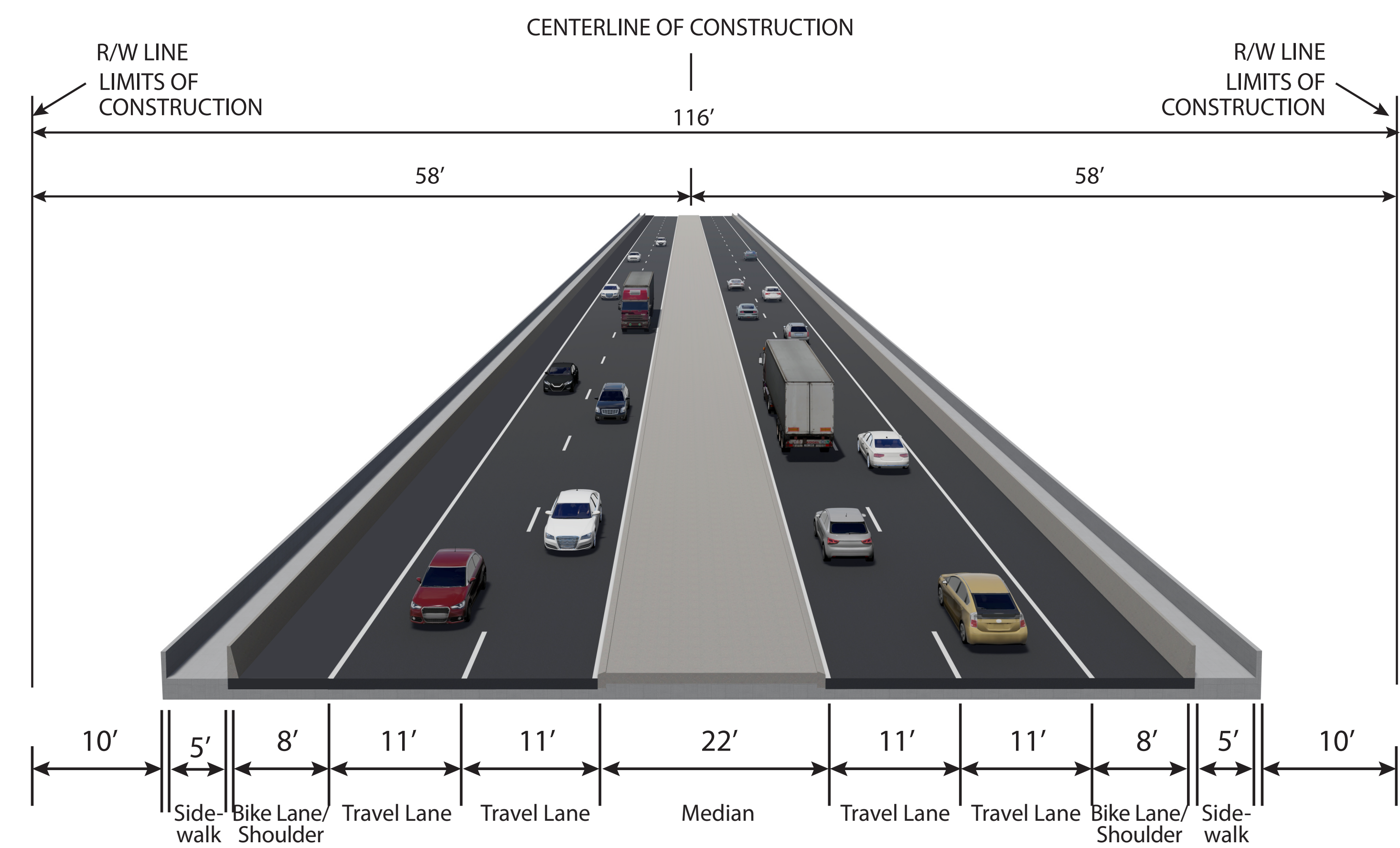
Typical Section on Bridge
