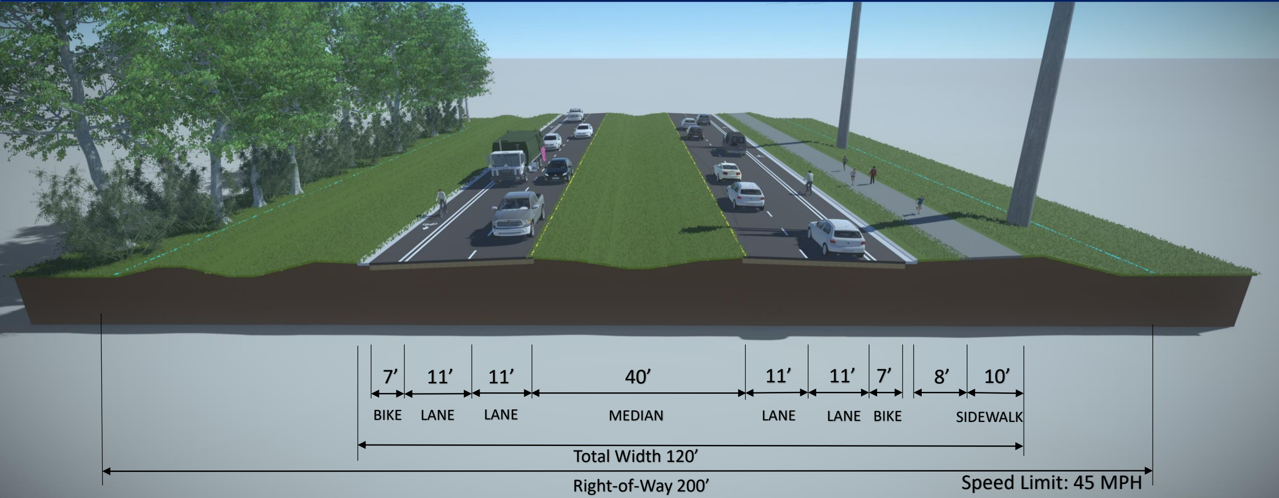
Preferred Typical Section
