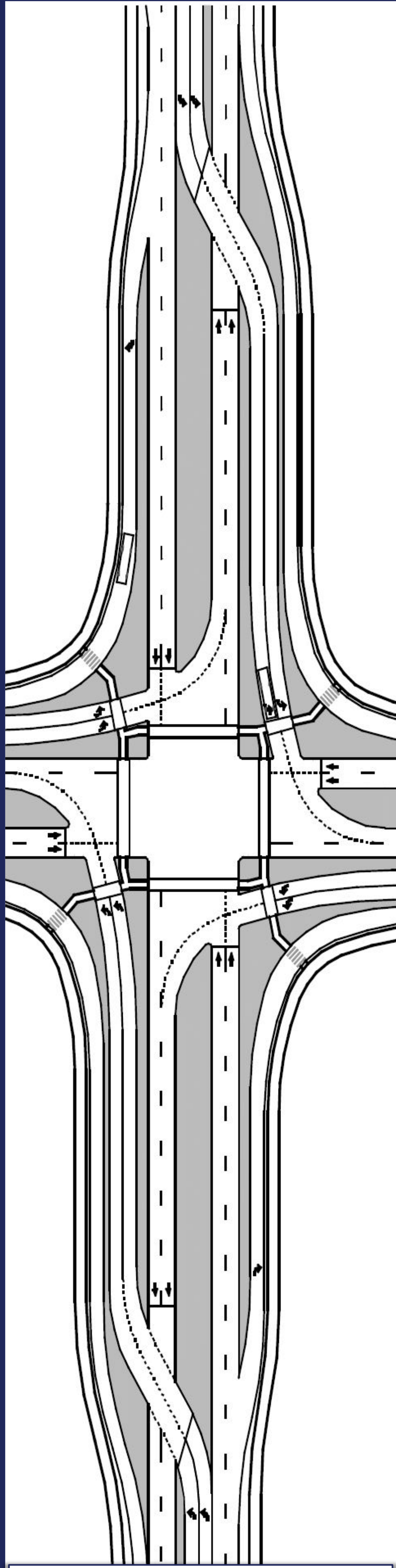
Example of Displaced Left Turn Alternative
